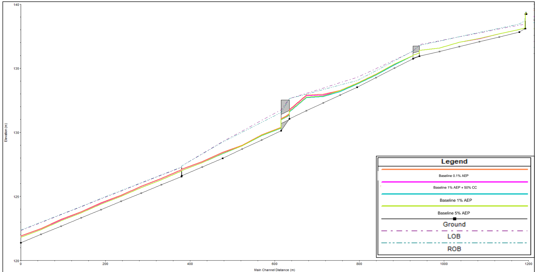
Figure 4.9: All AEP maximum baseline water levels – Hilton Park watercourse
