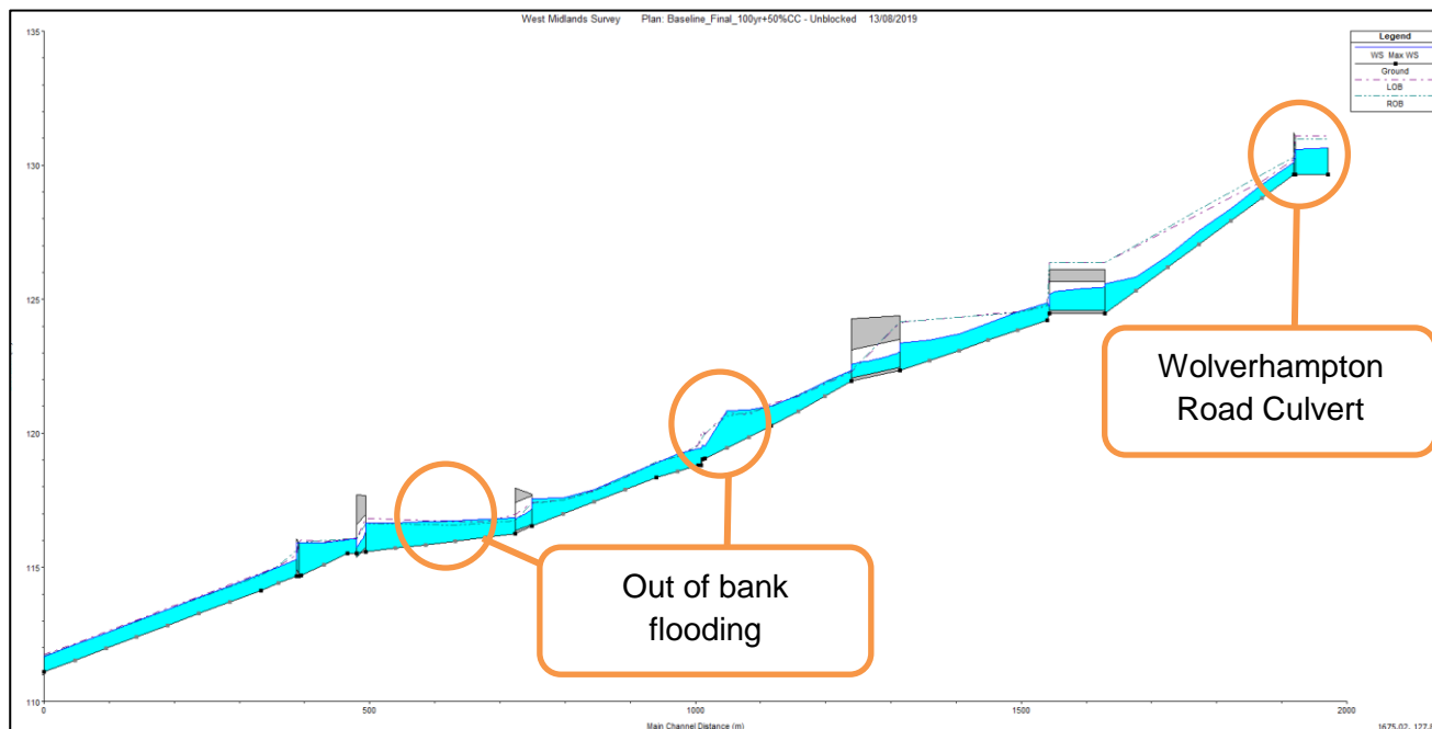
Figure 4.23: 1% AEP + 50% climate change allowance maximum water levels without culvert blockage long section
