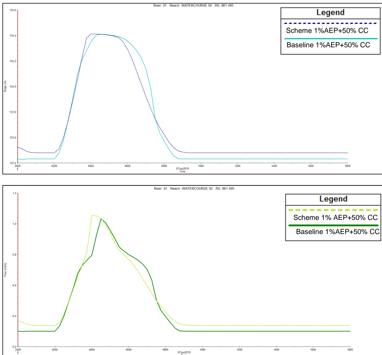
Figure 5.6: Comparison of peak stage and flow during a 1% AEP + 50% climate change event between baseline and scheme models
