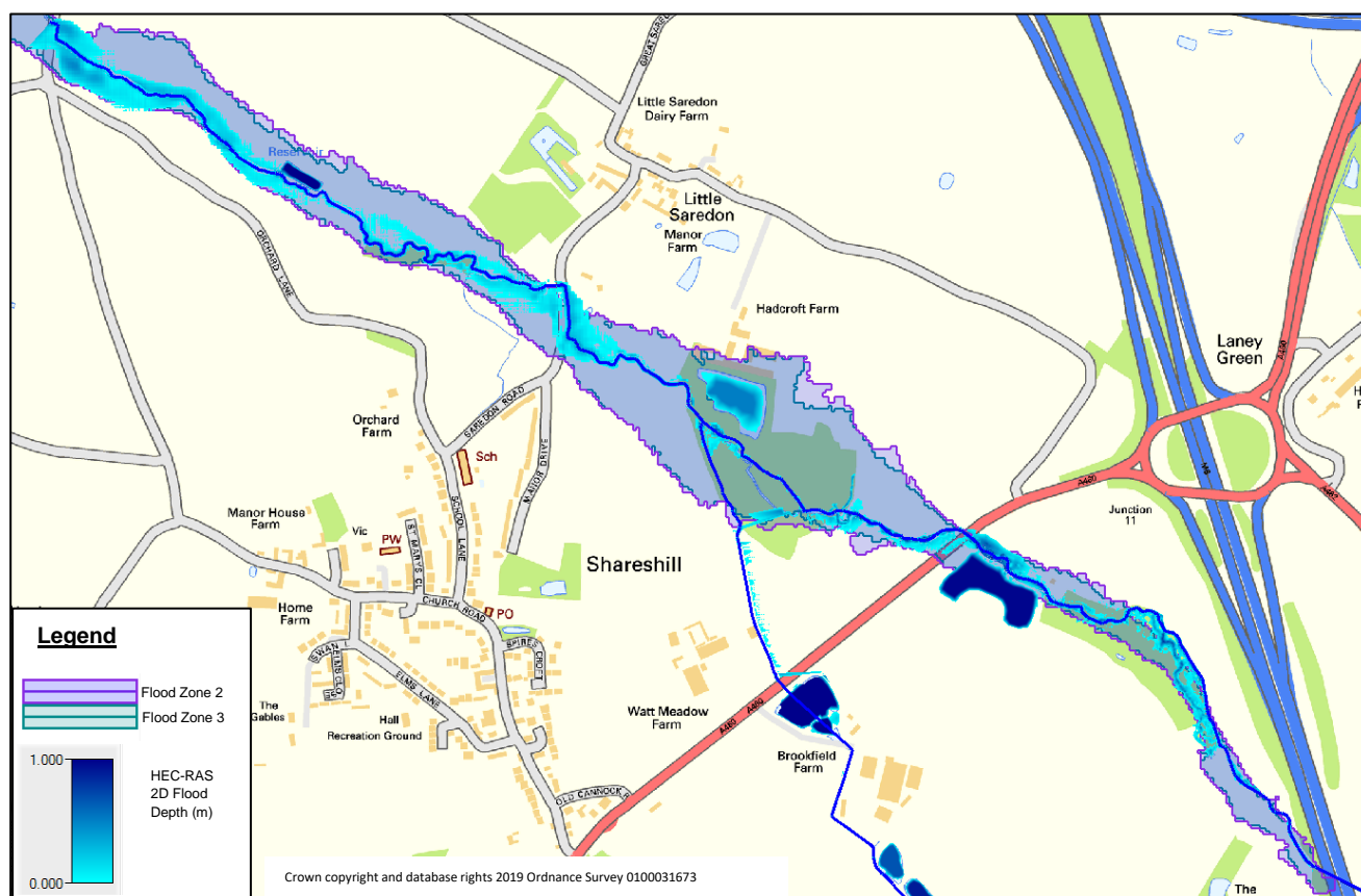
Figure 3.4: Environment Agency JFLOW model Flood Zone 2 and 3 outlines compared to Latherford Brook HEC-RAS model results for 1% AEP event
