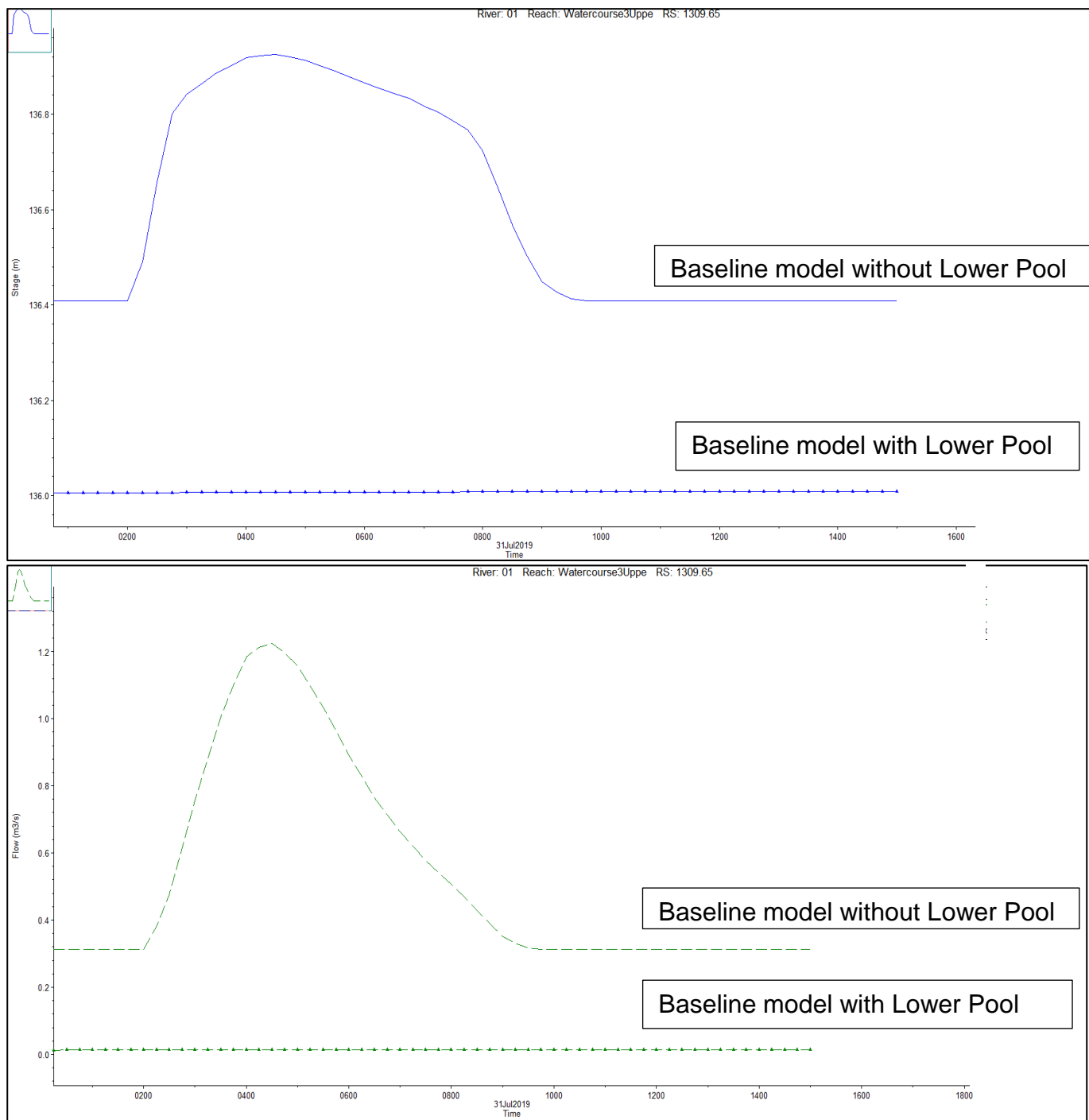
Figure 4.11: Sensitivity test stage and flow results for 1% AEP + 50% climate change allowance event showing the impact of exclusion of Lower Pool from the model.
