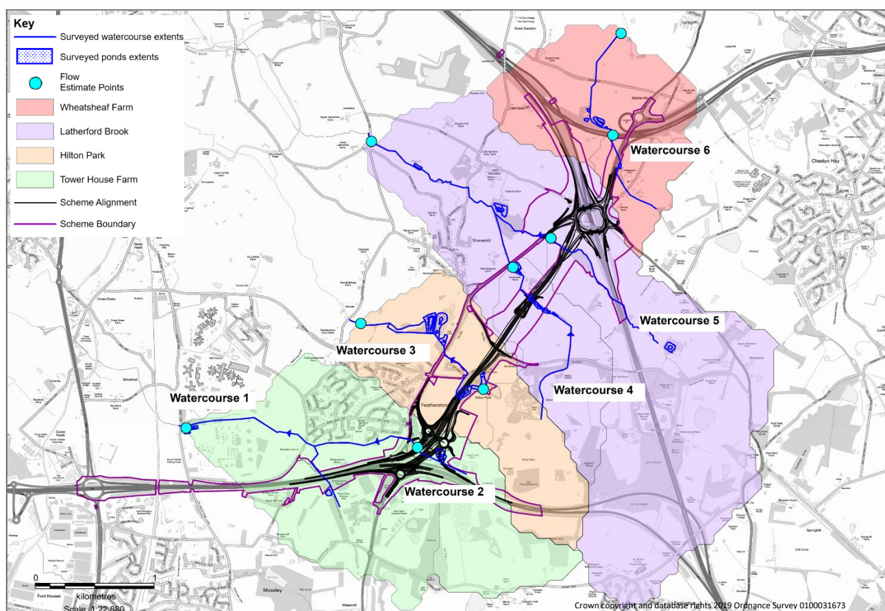
Figure 3.2: HEC-RAS modelling approach and flow estimation points
