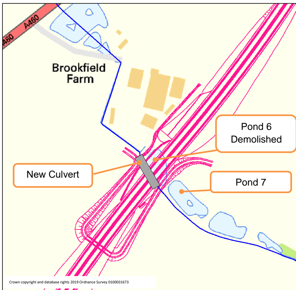
Figure 5.12: Watercourse 4 general scheme arrangement. Scheme alignment is shown in pink.
