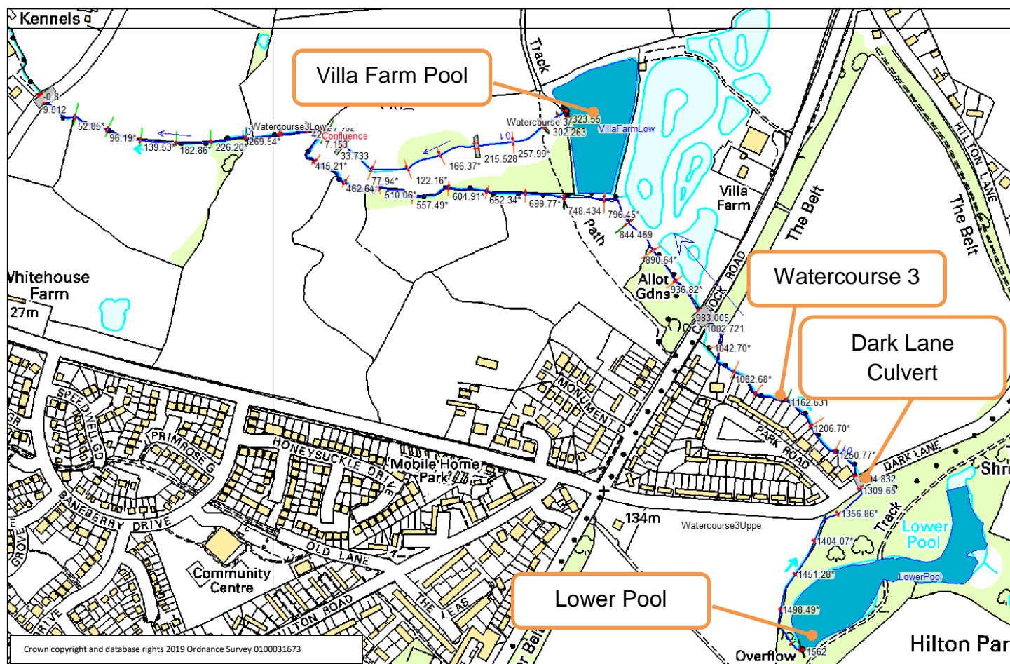
Figure 4.8: Overview of Hilton Park model extents
